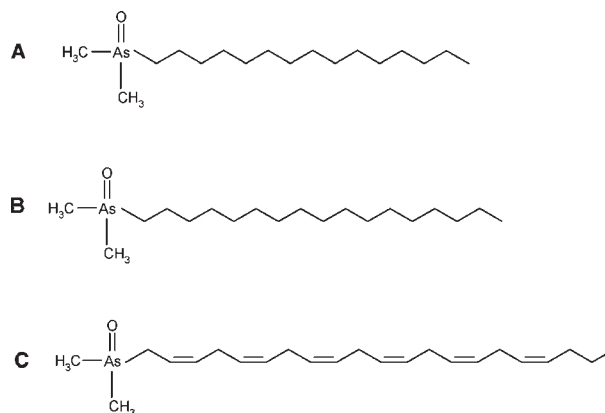
Fig. 1 Arsenic-containing hydrocarbons identified in oil from capelin. Assignments were based on high resolution accurate mass spectrometry, and, for compound A, confirmed by chemical synthesis. The position and geometry of the double bonds in compound C were not determined; they have been assigned by analogy to all-cis -4,7,10,13,16,19-docosahexaenoic acid [DHA, 22:6 ( n = 3)], a common fatty acid in fish.
